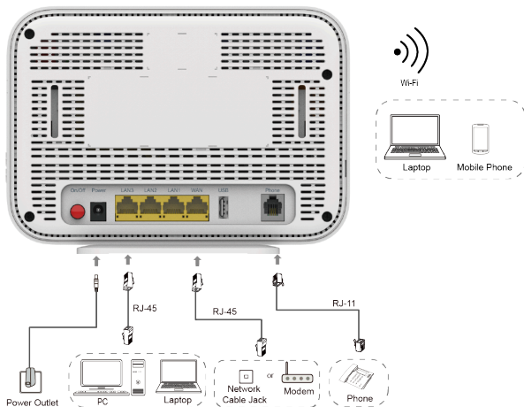
Figure 5-1 Cable Connection
