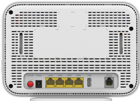
Figure 4-3 The Rear Panel
