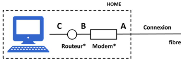
Figure 2: NTP localisation for internet service access (A=R/S and B = U), source IBPT
